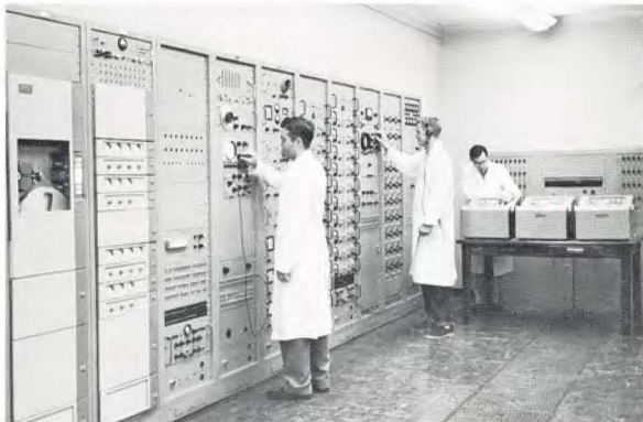
Seven-track FR-100A Recorder/Reproducer used for production-line testing of Jupiter missiles at Army Ballistic Missile Agency, Huntsville, Alabama. Photo courtesy Electrical Manufacturing Magazine
